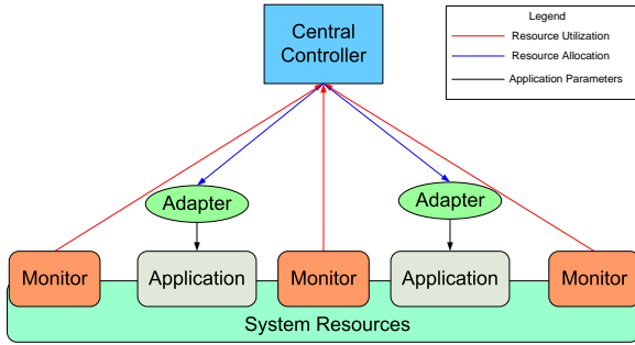
Figure 2: HyARM Architecture
