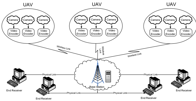
Figure 1: DRE Multimedia System Architecture
