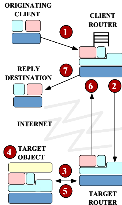
Figure 2: Store-and-Forward CORBA Twoway Request/Response via TII
