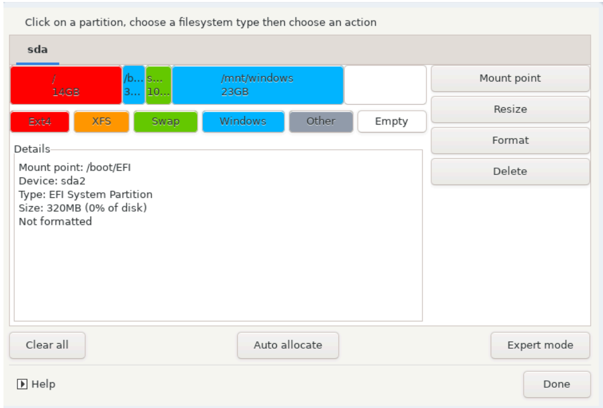
Figure 1. EFI System Partition
